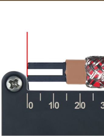
4: Graduated scale in cm, engraved, with mechanical stop at 0 cm , to ease the stripping length measurement.
