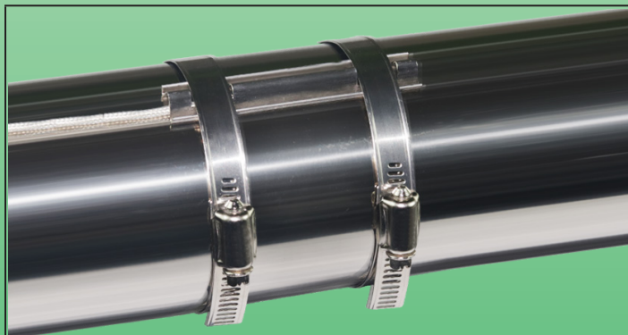
Example of the temperature sensor model after installation
